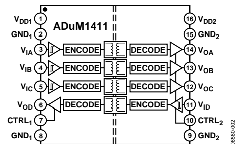
图2. ADuM1411
