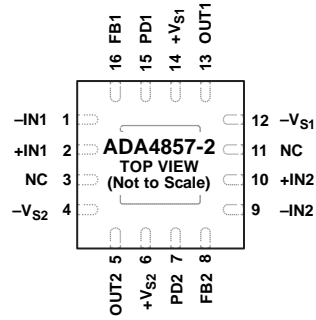
Figure 7. 16-Lead LFCSP Pin Configuration
