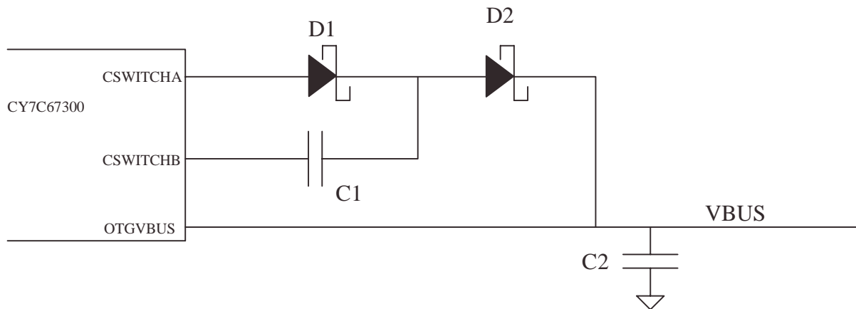
Figure 4-5. Charge Pump
