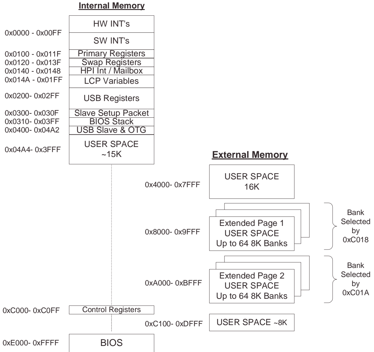
Figure 6-1. Memory Map
