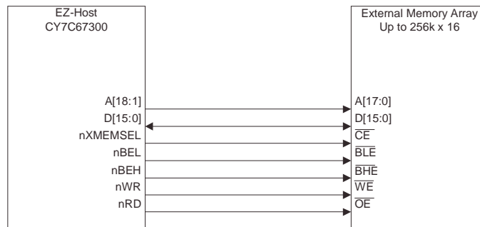
Figure 4-3. Interfacing up to 256k x 16 for External Code/Data
