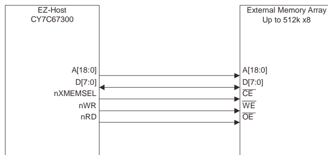
Figure 4-4. Interfacing up to 512k x 8 for External Code/Data
