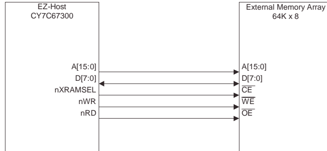
Figure 4-2. Interfacing to 64k x 8 Memory Array
