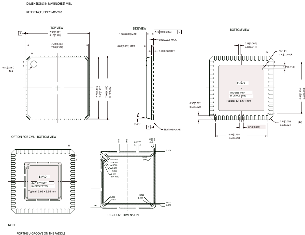
Figure 6. 56-Lead QFN 8 x 8 MM LF56A.
