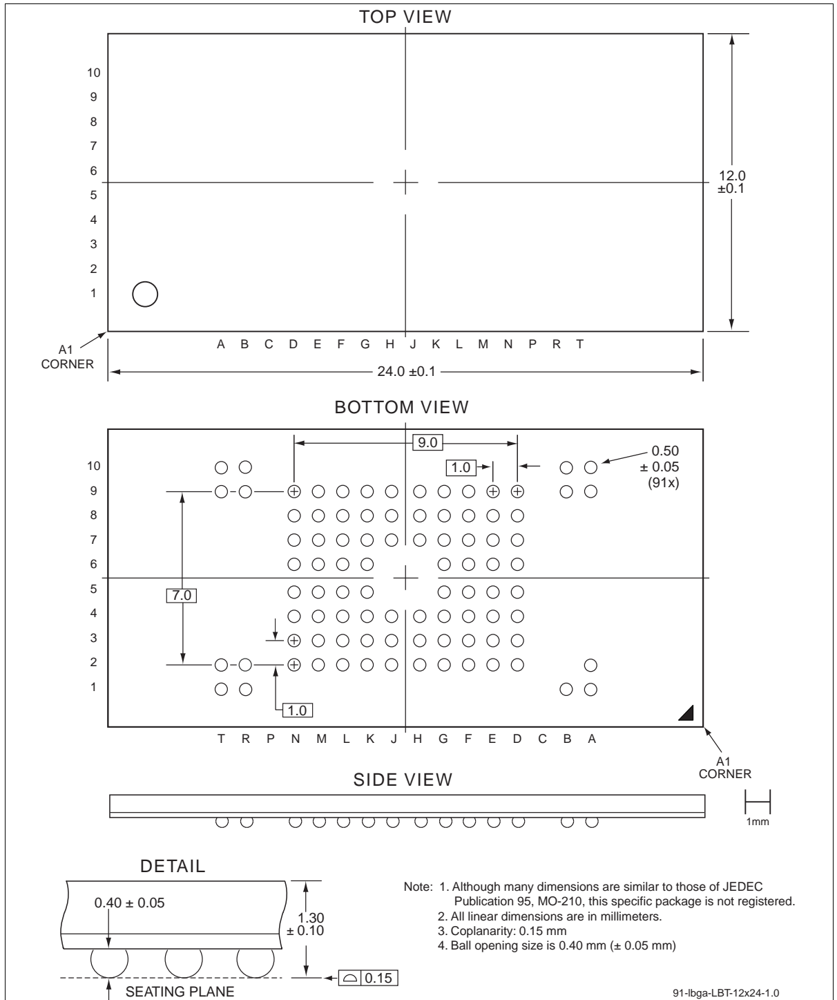
Figure 5: NANDrive 91-Ball, Low-profile Ball Grid Array (LBGA) Greenliant Package Code: LBT
