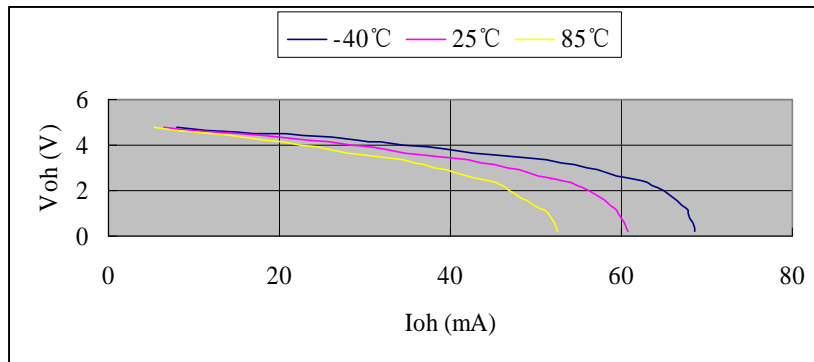
C: V_{OH} vs. I_{OH} @VDD = 5.5V
