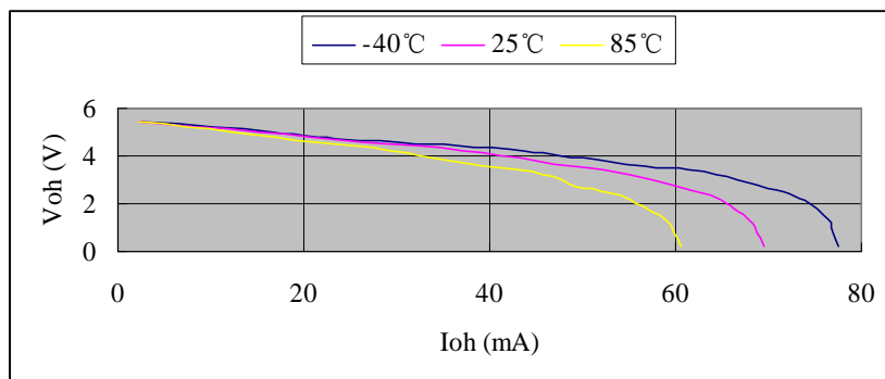
C: V_{OH} vs. I_{OH} @VDD = 5.5V
