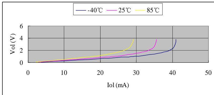
E: V_{OL} vs. I_{OL} @VDD = 5.0V
