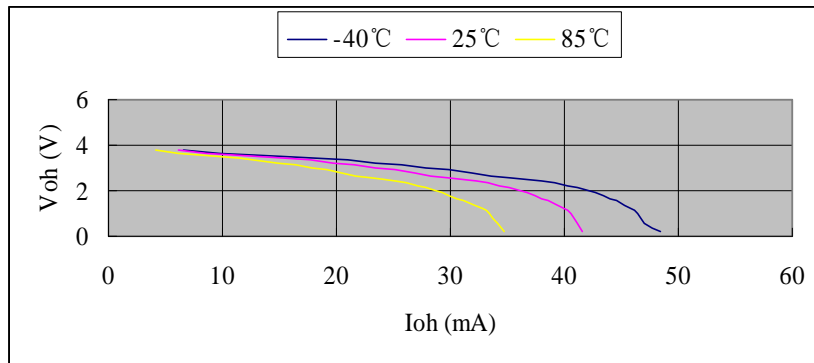
B: V_{OH} vs. I_{OH} @VDD = 5.0V
