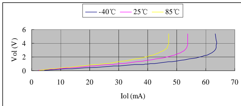
F: V_{OL} vs. I_{OL} @VDD = 5.5V
