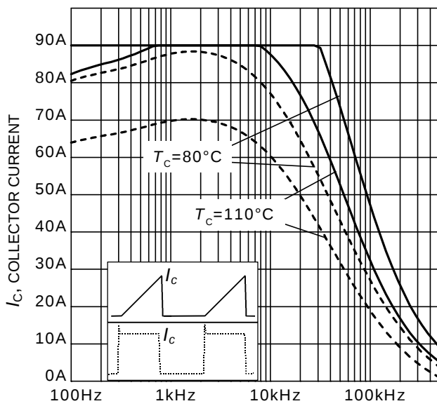
Figure 1. Collector current as a function of switching frequency ( T_j \leq 175^\circ\text{C} , D = 0.5 , V_{CE} = 400\text{V} , V_{GE} = 0/+15\text{V} , R_G = 10\Omega )
