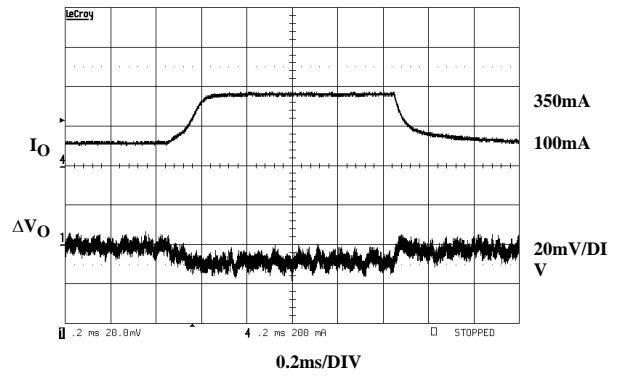
FIGURE 8. TRANSIENT RESPONSE
