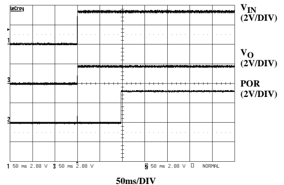
FIGURE 6. START-UP 2
