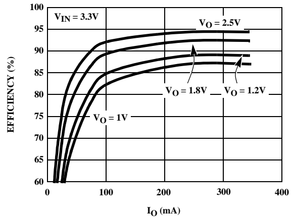
FIGURE 2. EFFICIENCY
