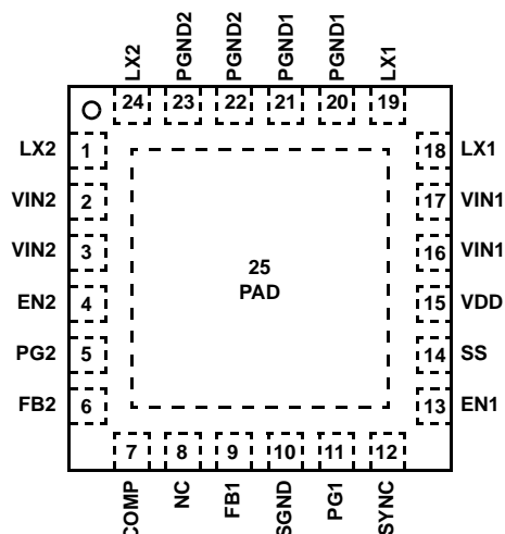
ISL8036, ISL8036A (24 LD QFN) TOP VIEW
