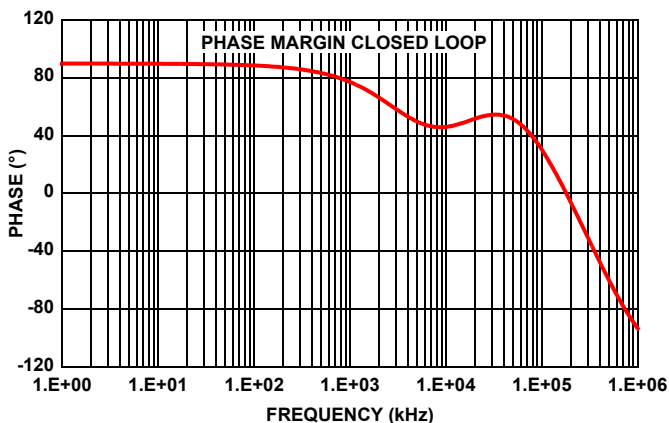
FIGURE 49. SIMULATED LOOP GAIN
