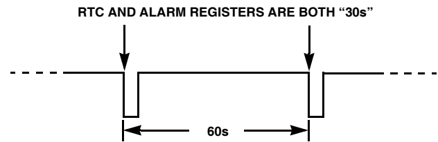
FIGURE 13. \overline{\text{IRQ}}/\text{F}_{\text{OUT}} WAVEFORM
