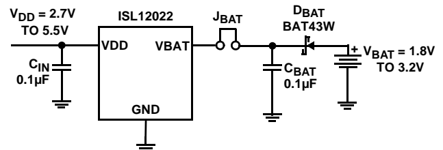
FIGURE 18. SUGGESTED BATTERY-BACKUP CIRCUIT
