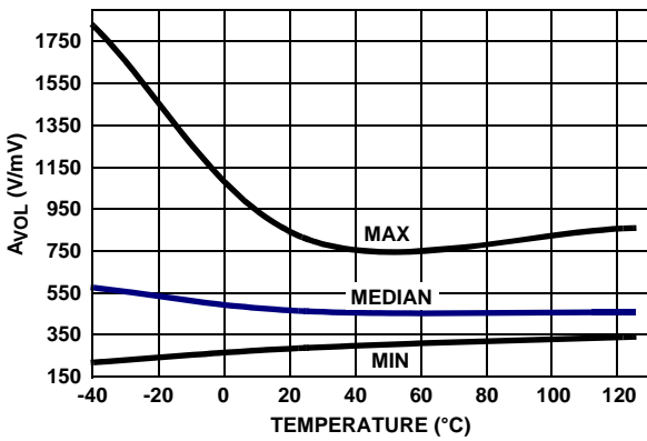
FIGURE 34. A_{VOL} vs TEMPERATURE R_L = 100k, V_+, V_- = \pm 2.5V, V_O = -2V \text{ TO } +2V
