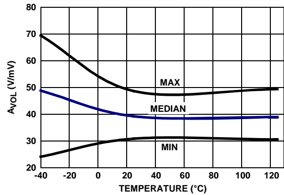
FIGURE 35. A_{VOL} vs TEMPERATURE R_L = 1k, V_+, V_- = \pm 2.5V, V_O = -2V \text{ TO } +2V
