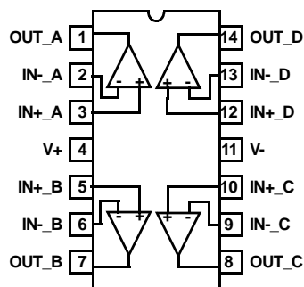
ISL28448 (14 LD TSSOP) TOP VIEW
