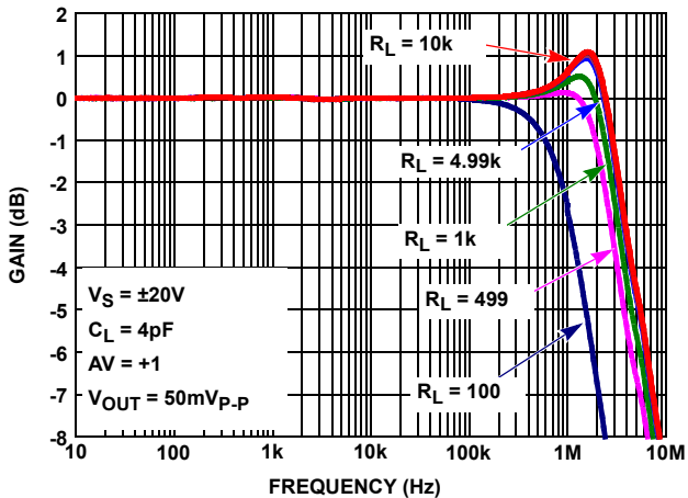
FIGURE 61. CHARACTERIZED CLOSED LOOP GAIN vs R_L
