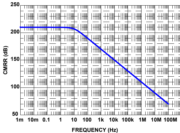
FIGURE 67. SIMULATED CMRR vs FREQUENCY
