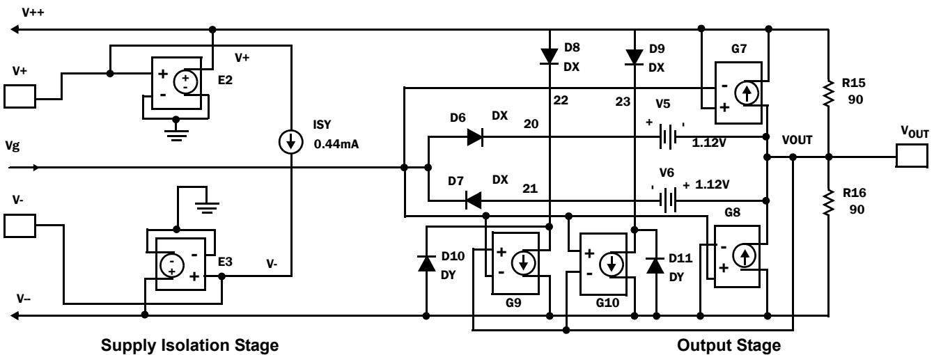
FIGURE 55. SPICE SCHEMATIC
