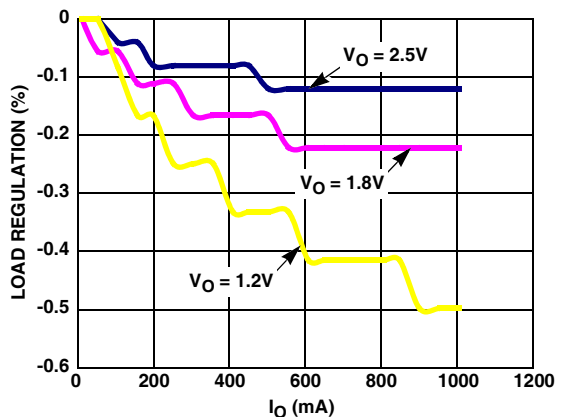
FIGURE 4. LOAD REGULATION vs I_O AT 3.3V V_{IN}
