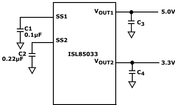
FIGURE 39. INDEPENDENT START-UP
