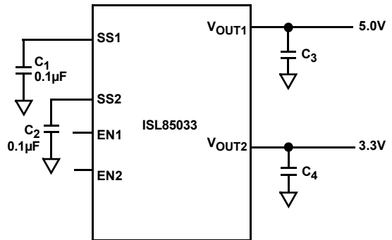
FIGURE 42. OUTPUT SEQUENCING
