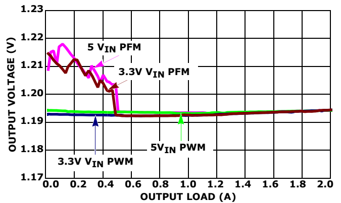
FIGURE 8. V_{OUT} REGULATION vs LOAD, 2.25MHz, 1.2V, CHANNEL1
