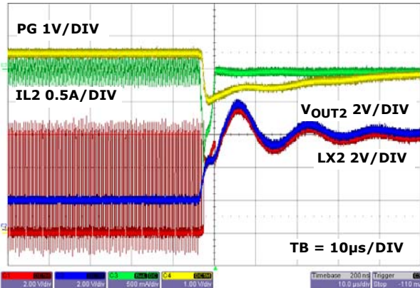
FIGURE 38. V_{OUT2} HARD SHORT TO V_{IN} NEGATIVE CURRENT WAVEFORMS AT HIGH LINE CHANNEL 2
