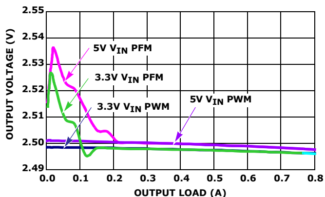
FIGURE 10. V_{OUT} REGULATION vs LOAD 2.25MHz 2.5V OUT
