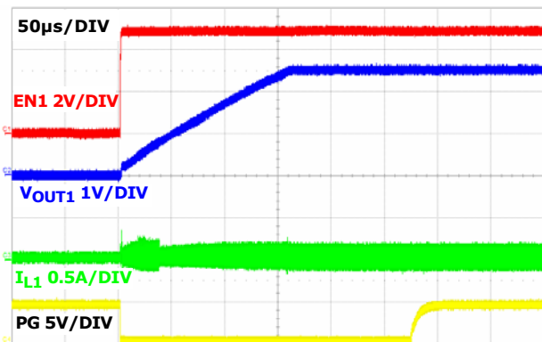
FIGURE 24. SOFT-START WITH NO LOAD CHANNEL 1 (PWM)
