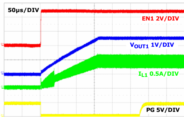
FIGURE 28. SOFT-START AT FULL LOAD CHANNEL 1
