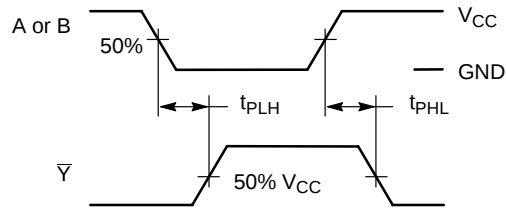
Figure 3. Switching Waveform
