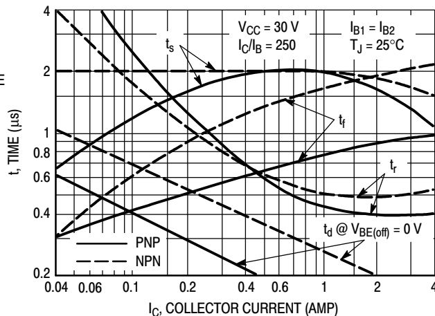
Figure 2. Switching Times
