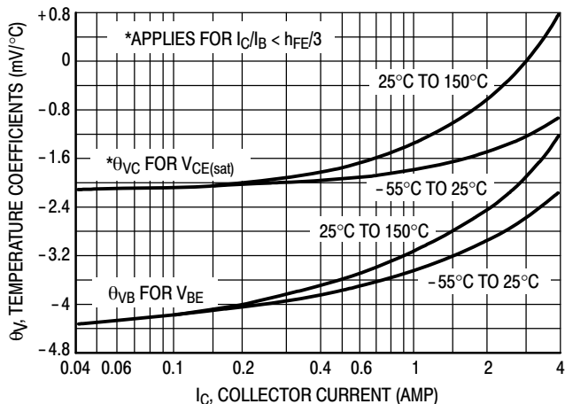
Figure 10. Temperature Coefficients
