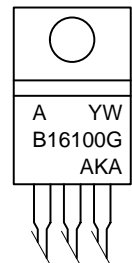
TO-220AB CASE 221A PLASTIC
