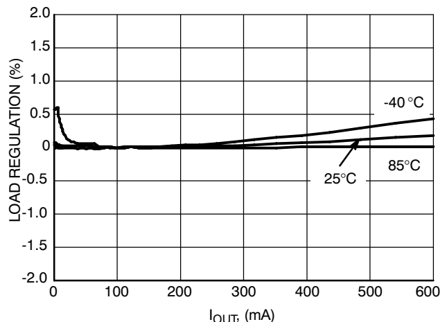
Figure 30. Load Regulation (V IN = 5.0 V, V OUT = 3.9 V)
