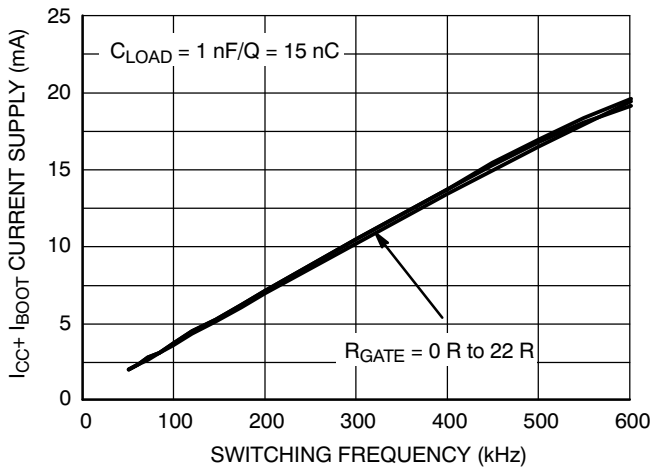
Figure 44. I_{CC1} Consumption vs. Switching Frequency with 15 nC Load on Each Driver @ V_{CC} = 15 V
