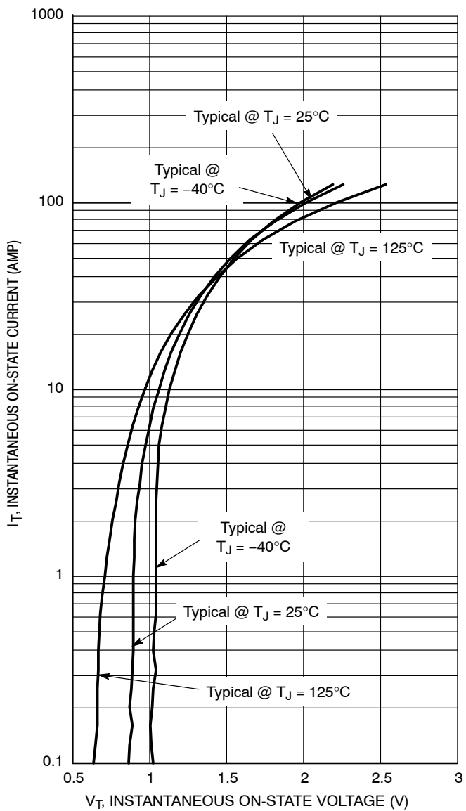
Figure 3. On-State Characteristics
