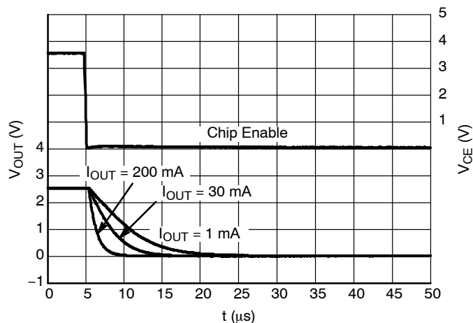
Figure 44. Shutdown, 2.5 V Version D, V_{IN} = 3.5 V
