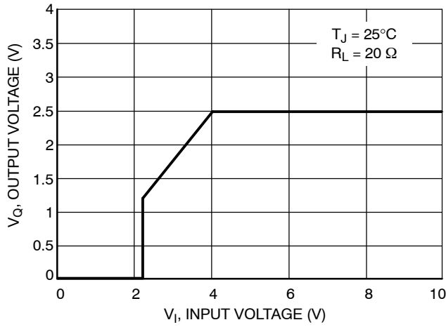
Figure 18. Low Voltage Behavior, Adjustable Version
