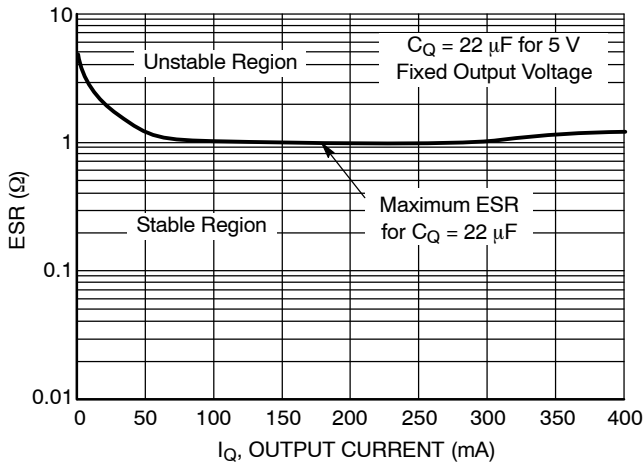
Figure 5. Output Stability with 22 \mu\text{F} Output Capacitor ESR, 5.0 V Regulator
