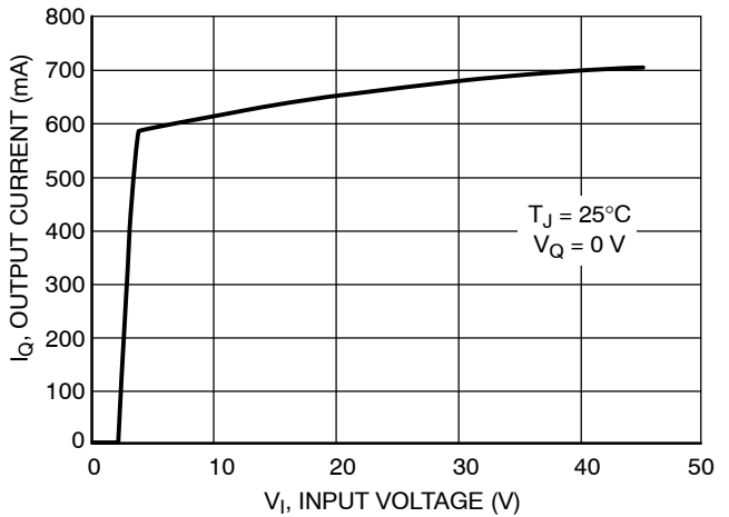
Figure 21. Maximum Output Current vs. Input Voltage, Adjustable Version
