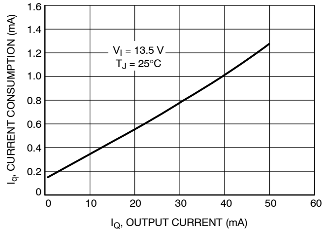
Figure 15. Current Consumption vs. Output Current (Low Load)
