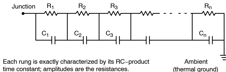
Figure 26. Non-Grounded Capacitor Thermal Ladder ("Foster" Ladder)
