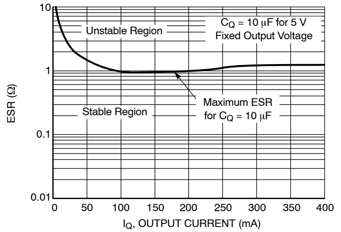
Figure 6. Output Stability with 10 \mu\text{F} Output Capacitor ESR, 5.0 V Regulator
