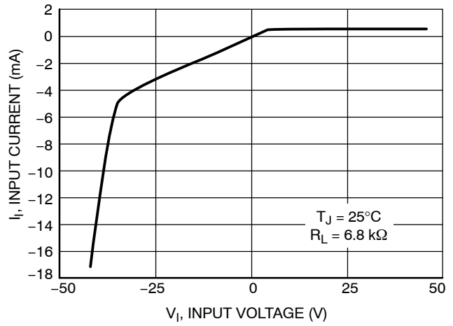
Figure 19. High Voltage Behavior, Adjustable Version
