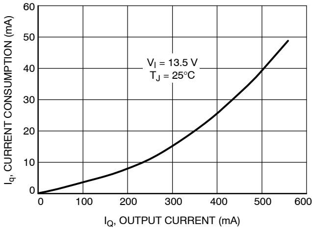
Figure 14. Current Consumption vs. Output Current (High Load)
