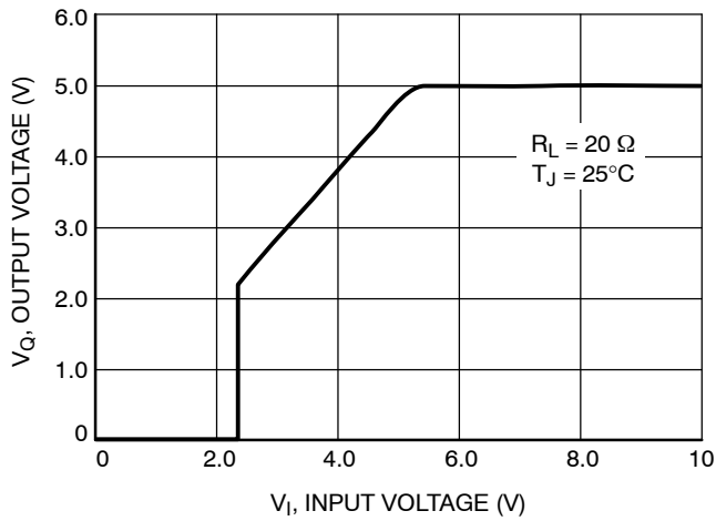
Figure 10. Low Voltage Behavior, 5.0 V Version
