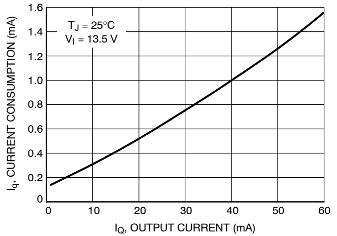
Figure 23. Current Consumption vs. Output Current (Low Load), Adjustable Version
