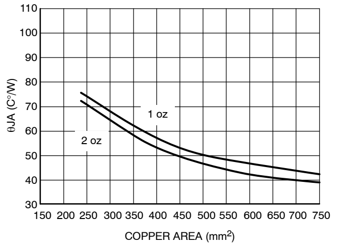
Figure 28. \theta_{JA} vs. Copper Spreader Area, D 2 PAK 5-Lead
