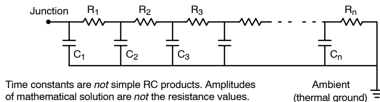
Figure 25. Grounded Capacitor Thermal Network ("Cauer" Ladder)
