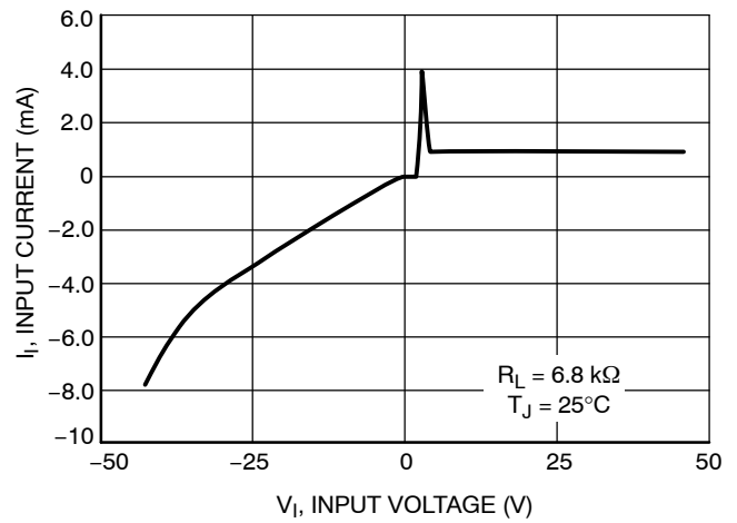
Figure 11. Input Current vs. Input Voltage, 5.0 V Version
