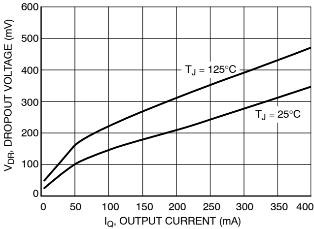
Figure 20. Dropout Voltage vs. Output Current, Regulator Set at 5.0 V, Adjustable Version
