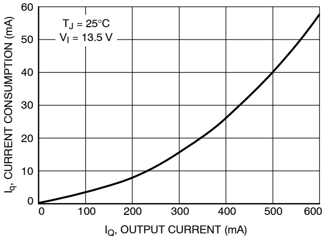
Figure 22. Current Consumption vs. Output Current (High Load), Adjustable Version
