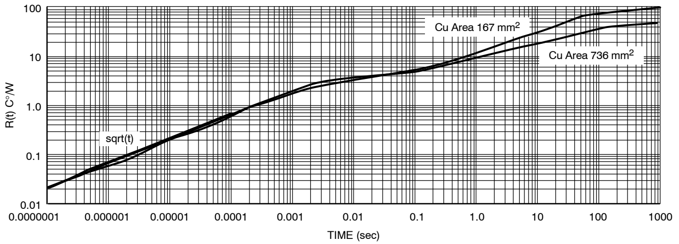
Figure 29. Single-Pulse Heating Curves, DPAK 5-Lead
