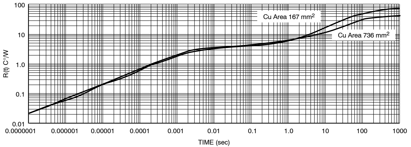
Figure 30. Single-Pulse Heating Curves, D 2 PAK 5-Lead
