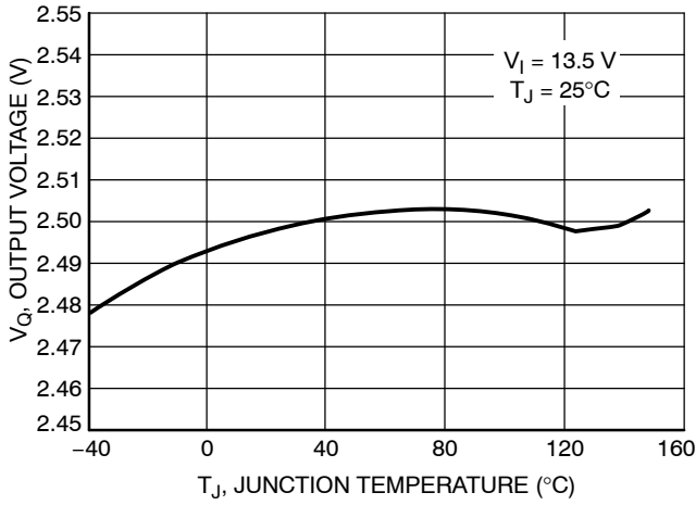
Figure 16. Output Voltage vs. Junction Temperature, Adjustable Version
