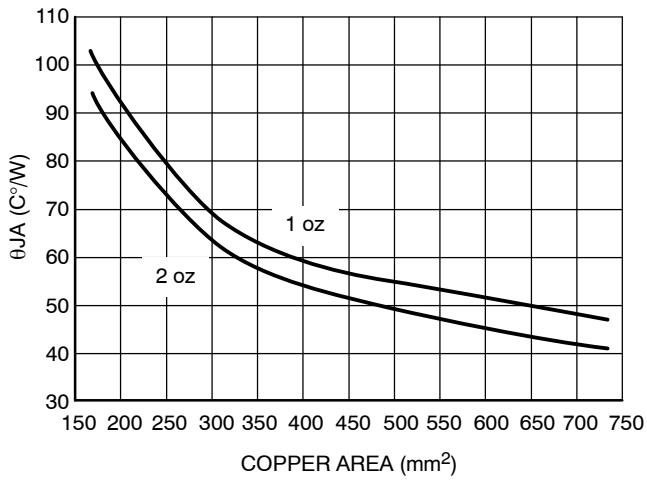
Figure 27. \theta_{JA} vs. Copper Spreader Area, DPAK 5-Lead
