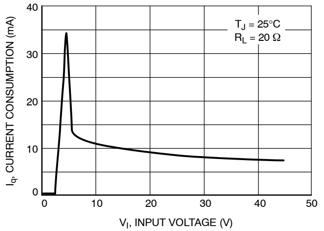
Figure 9. Current Consumption vs. Input Voltage, 5.0 V Version
