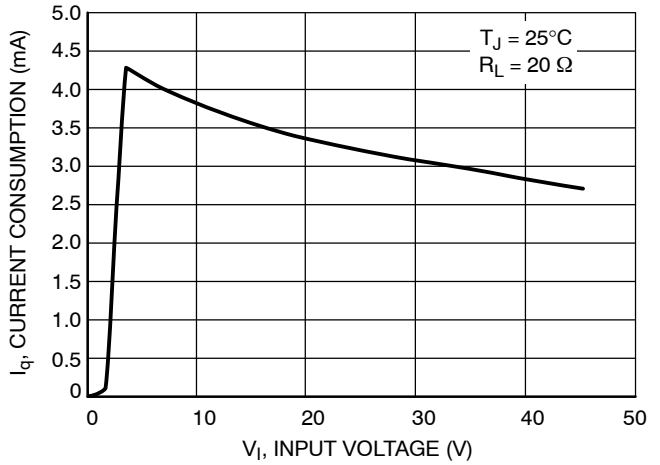
Figure 17. Current Consumption vs. Input Voltage, Adjustable Version
