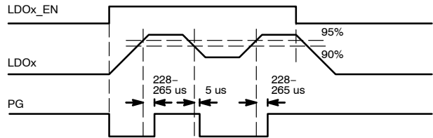
Figure 24. LDOx Channel Internal Power Good Signal
