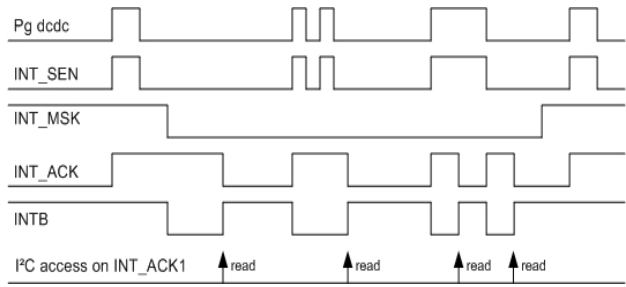
Figure 27. Interrupt Timing Chart Example of PG_DCDC
