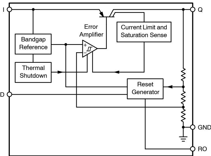
Figure 1. Block Diagram
