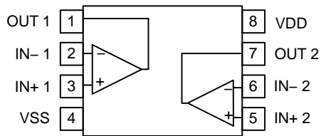
Dual Channel Configuration NCS2333, NCV2333
