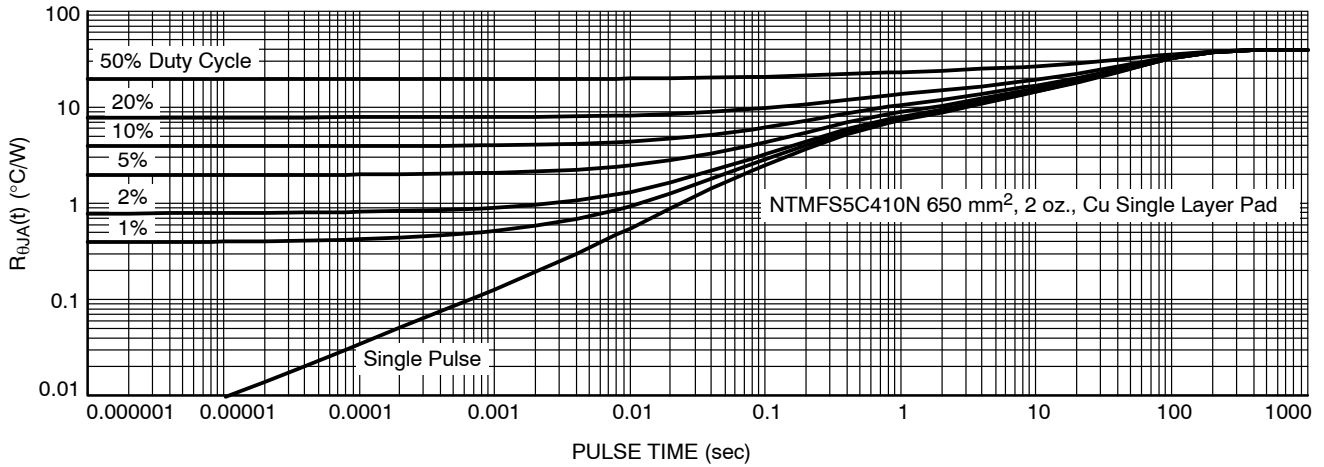
Figure 13. Thermal Characteristics – R_{\theta JA}(t) (°C/W)
