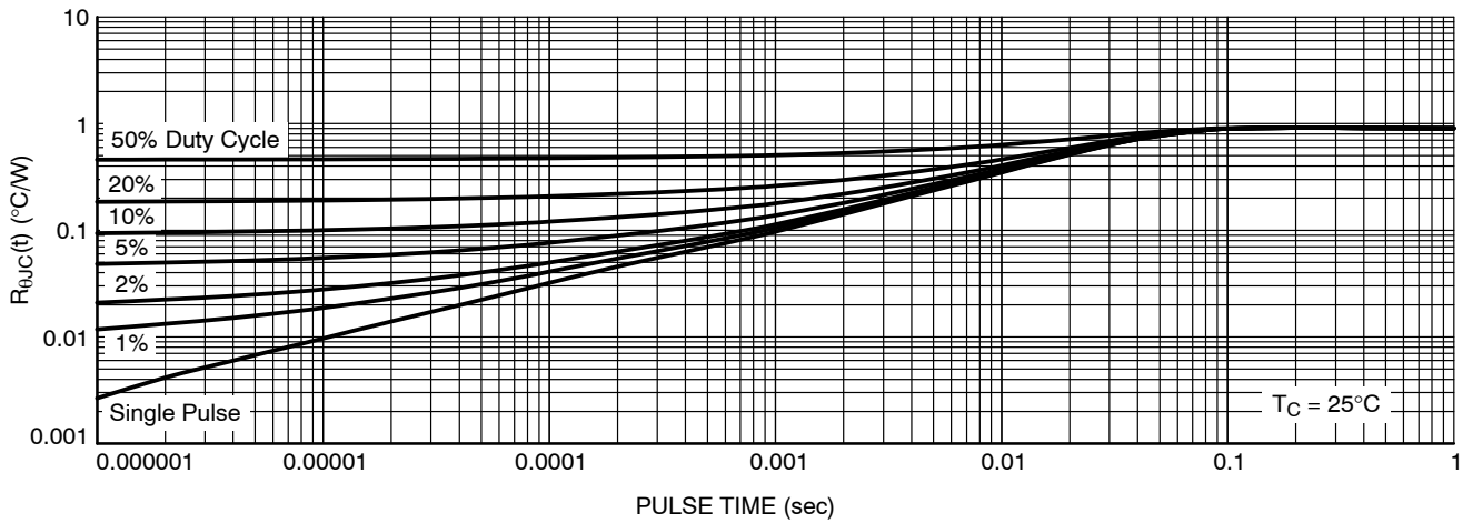
Figure 14. Thermal Characteristics – R_{\theta JC}(t) (°C/W)
