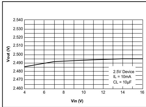
Figure 4. Line Regulation
