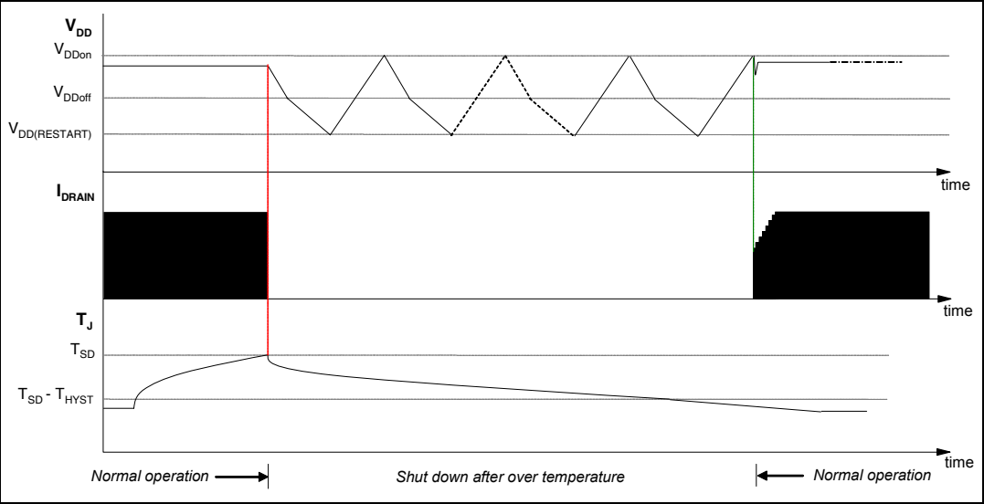
Figure 19. Thermal shutdown
