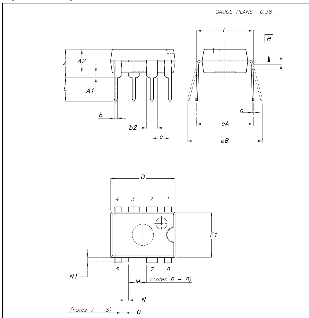
Figure 33. Package dimensions
