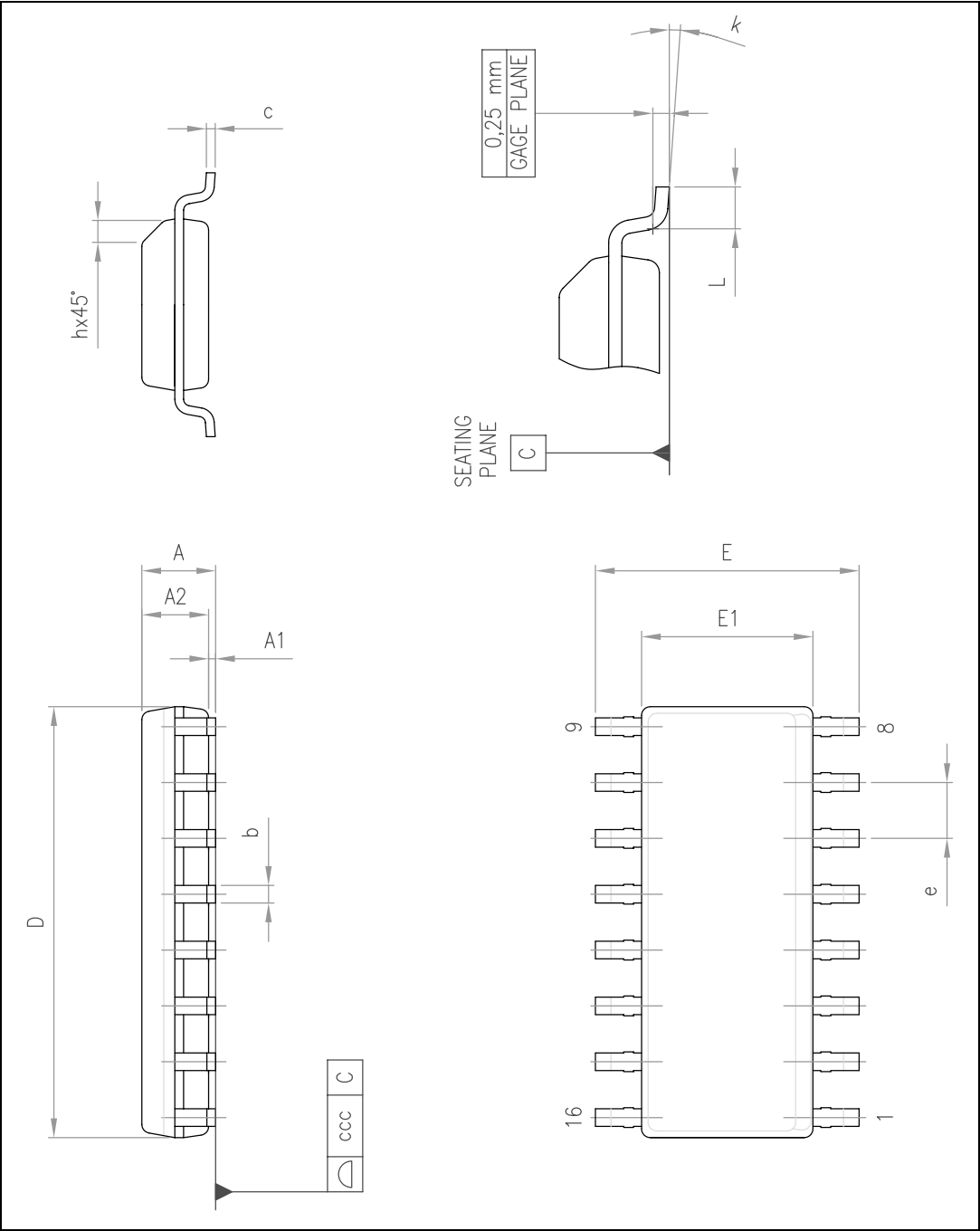
Figure 34. Package dimensions
