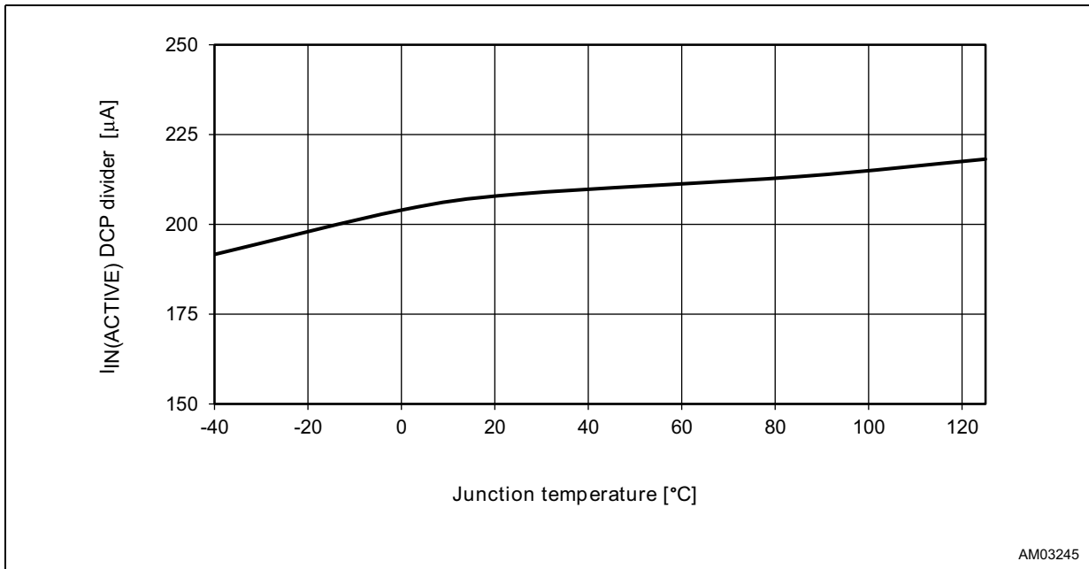
Figure 16. Enabled IN supply current vs. temperature (DCP divider mode)
