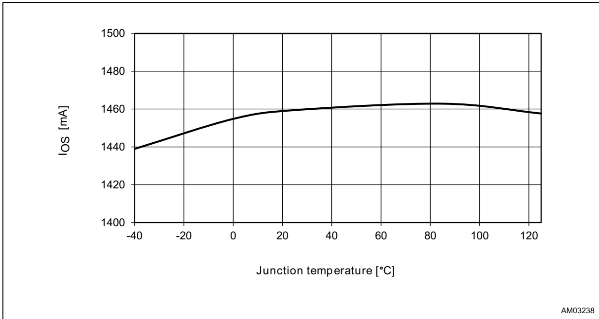
Figure 14. OUT short circuit current limit vs. temperature ( R_{LIM} = 33\text{ k}\Omega )
