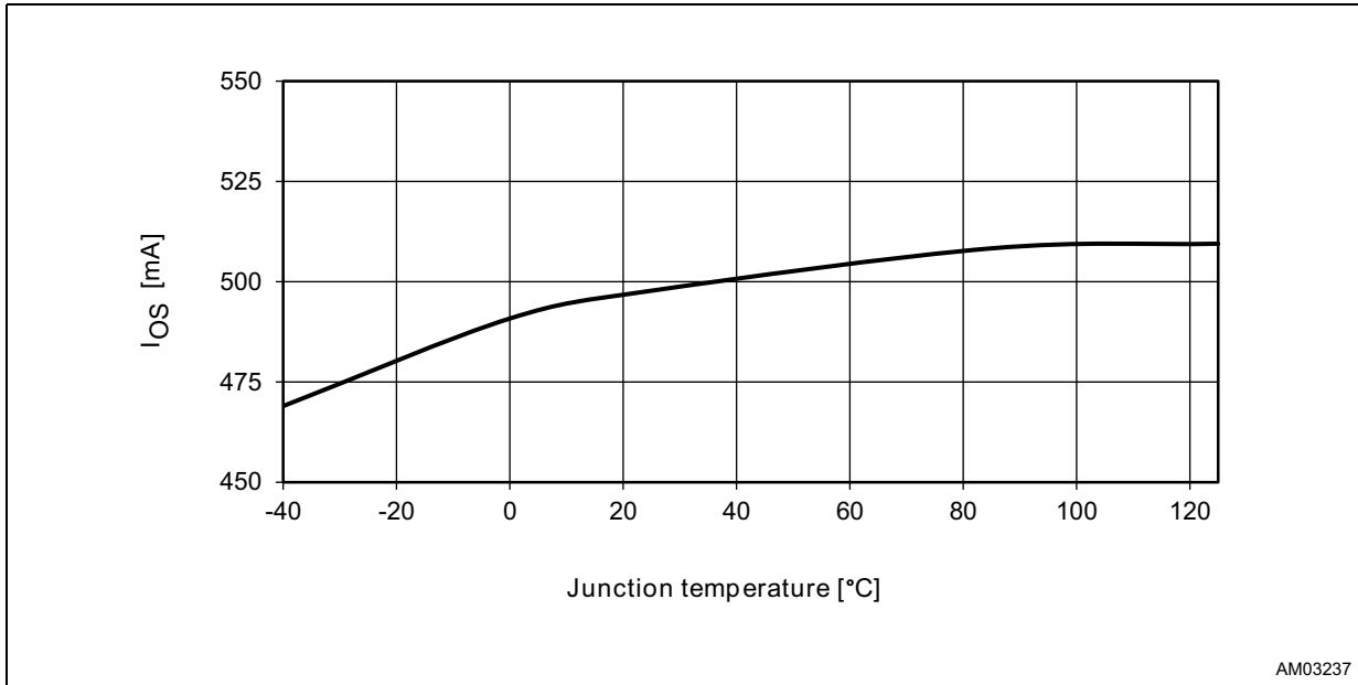
Figure 13. OUT short circuit current limit vs. temperature ( R_{LIM} = 96\text{ k}\Omega )
