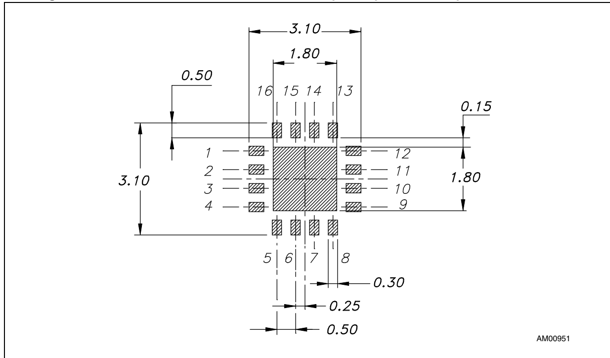
Figure 31. VFQFPN 16L - 3 x 3 x 0.8 mm with exposed pad 1.7 - footprint recommended
