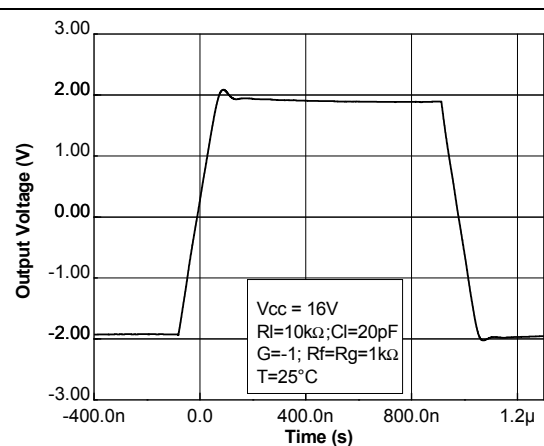
Figure 25. Large step response
