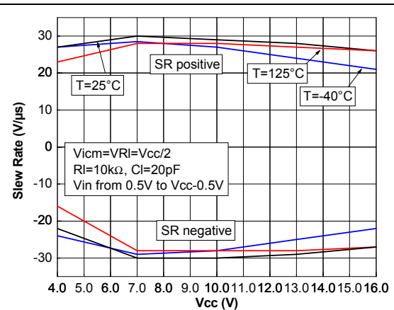
Figure 21. Slew rate vs. supply voltage and temperature
