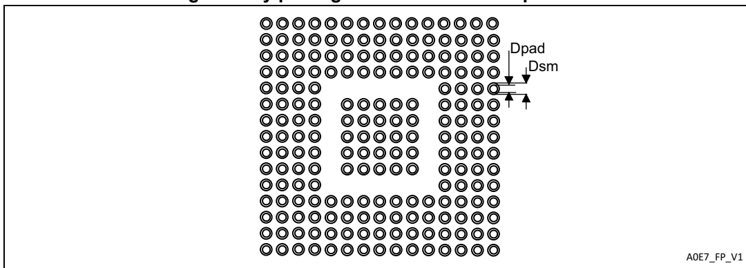
Figure 63. UFBGA176+25 - 201-ball, 10 x 10 mm, 0.65 mm pitch, ultra fine pitch ball grid array package recommended footprint
