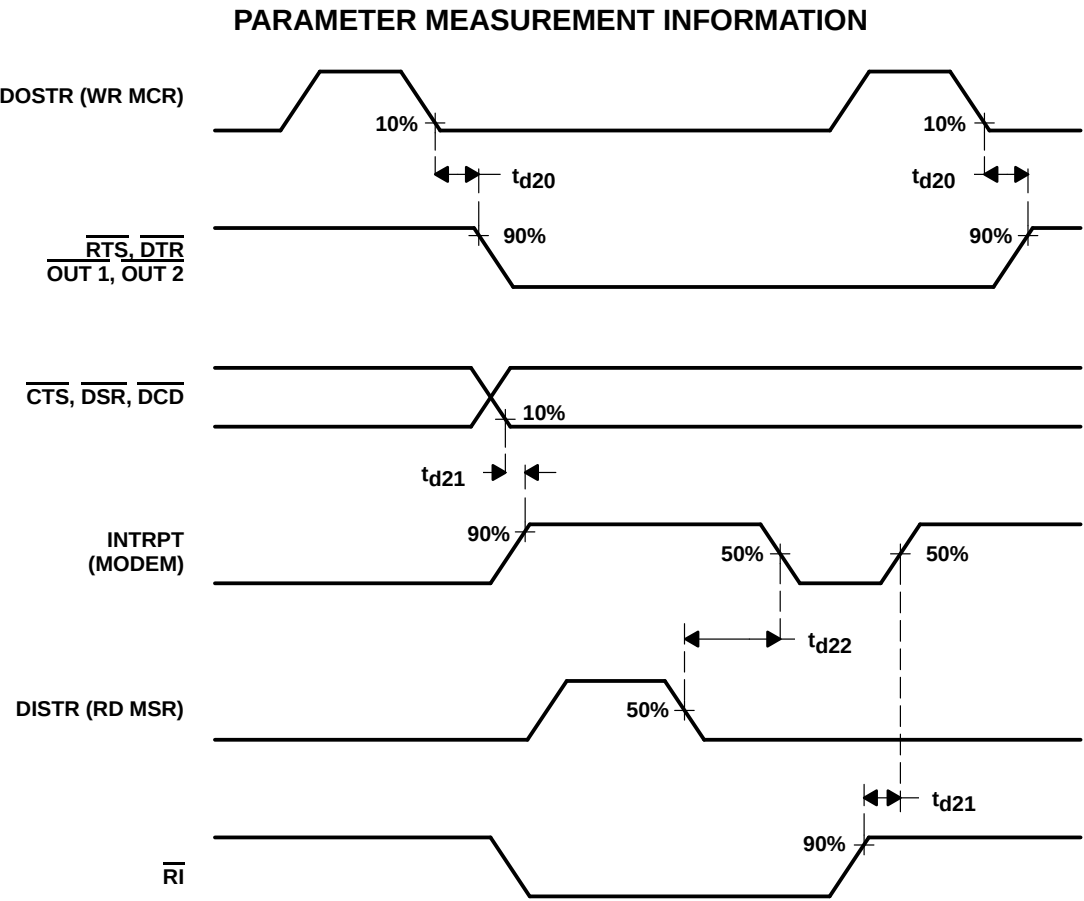
Figure 6. Modem Control Timing Waveforms
