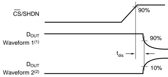
Voltage Waveforms for t_{dis}
