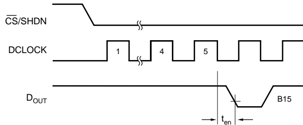
Voltage Waveforms for t_{en}
