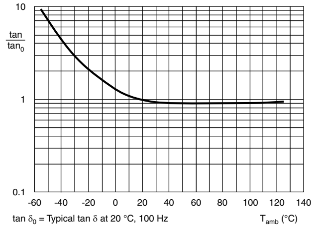
Fig. 7 - Typical multiplier of dissipation factor (tan δ) as a function of ambient temperature
