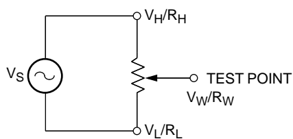
Test Circuit #1
