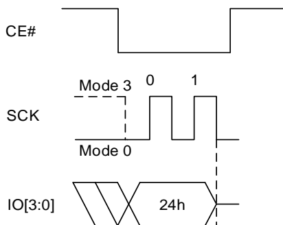
Figure 8.101 Sector Lock Sequence In QPI Mode
