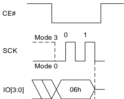
Figure 8.42 Write Enable Sequence In QPI Mode
