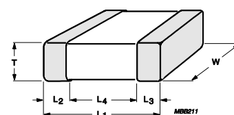
Fig. 2 Surface mounted multilayer ceramic capacitor dimension
