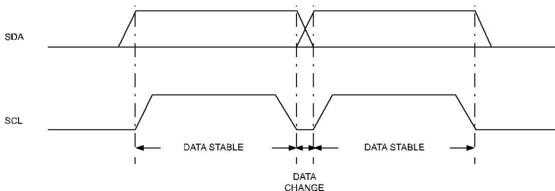
Figure 1. Data Validity
