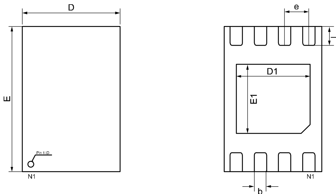
bottom view
