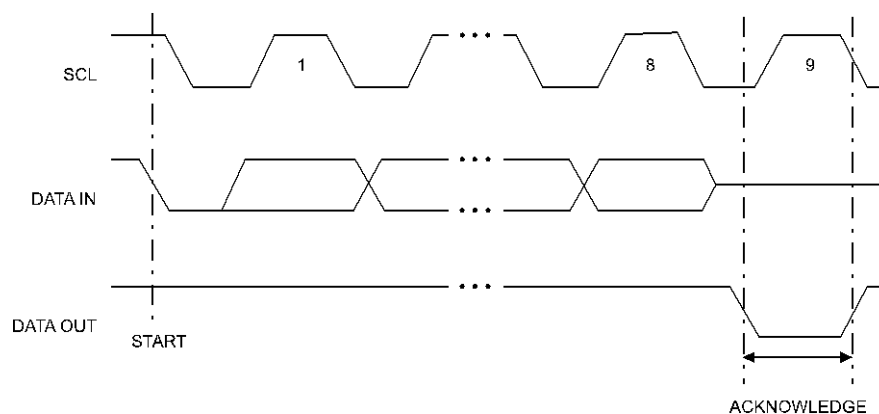
Figure 3. Output Acknowledge
