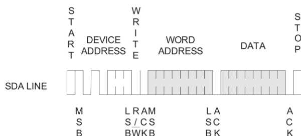
Figure 5. Byte Write
