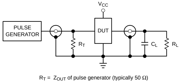
Figure 4. Test Circuit
