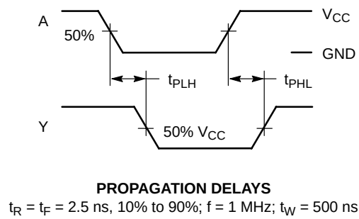
Figure 3. Switching Waveforms
