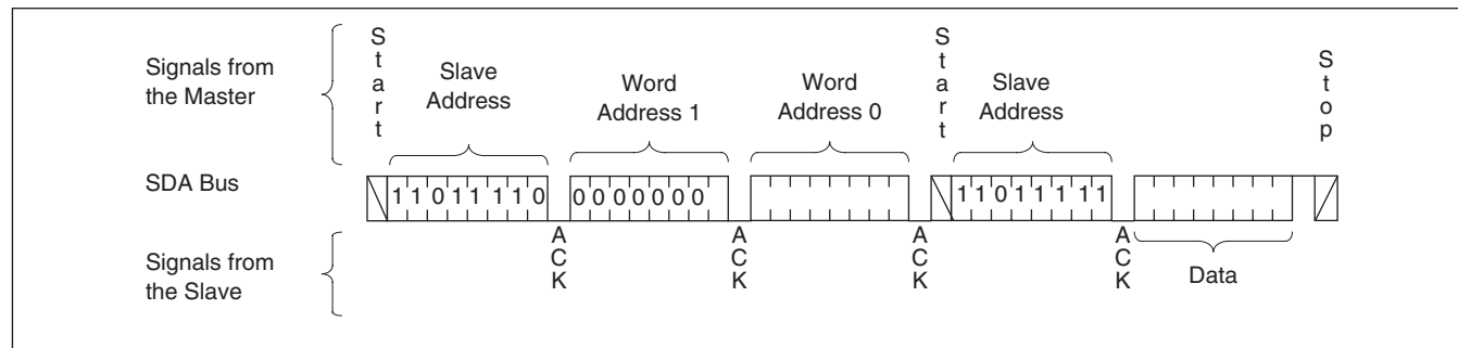
Figure 12. Sequential Read Sequence
