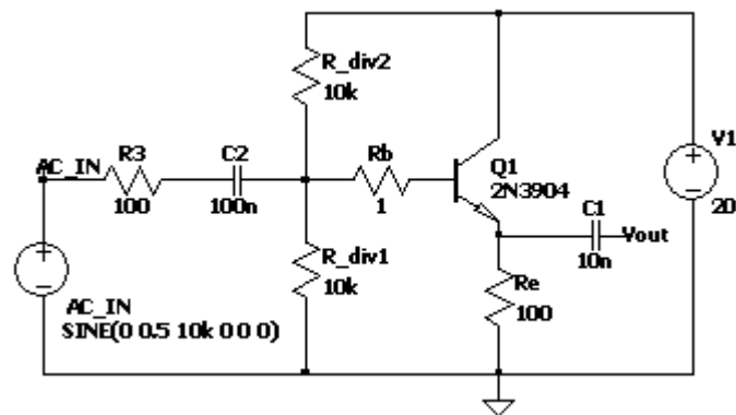
Common Collector
