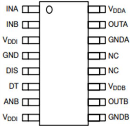
SOIC 16 Narrow
