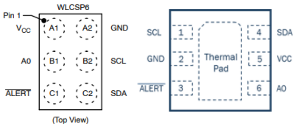
Pinout
