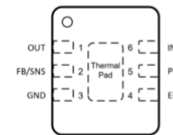
WDFNW6 2x2, 0.65P CASE 511DW
