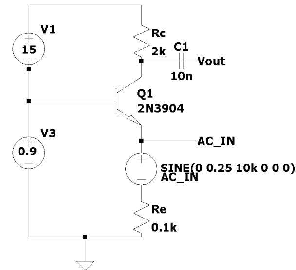
Common Base
