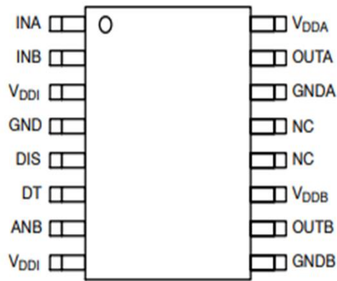
SOIC 16 Wide
