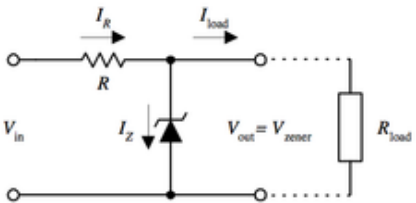
Voltage Regulator
