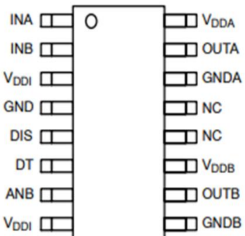
SOIC 16 Narrow
