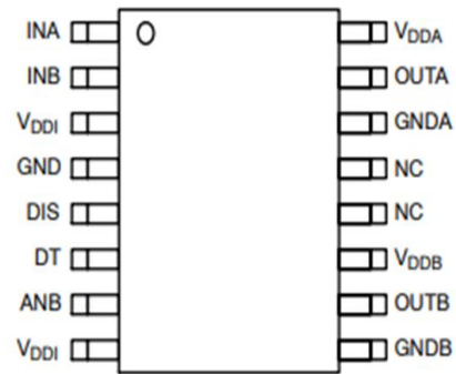
SOIC 16 Wide
