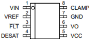
NCD(V)5701 / NCD(V)5703 A: Active Miller Clamp
