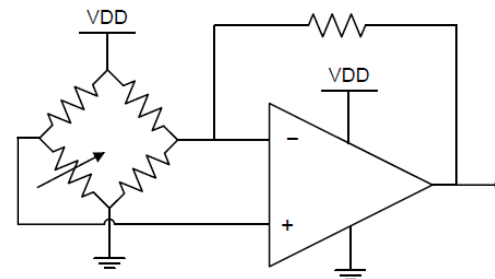
Figure 18. Bridge Circuit Amplification
