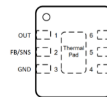
WDFNW6 2x2, 0.65P CASE 511DW
