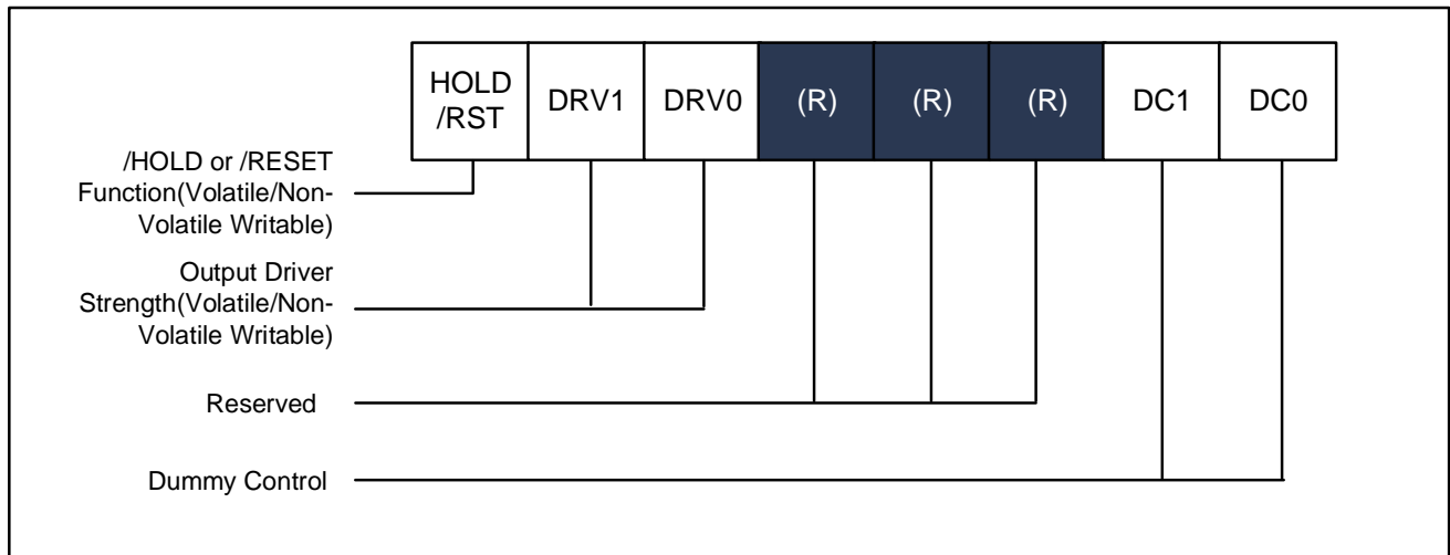
Figure 8-3 Status Register-3
