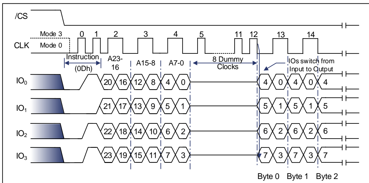
Figure 9-14 DTR Fast Read Instruction (QPI Mode)
