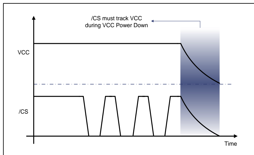
Figure 10-3 Power-Down Timing
