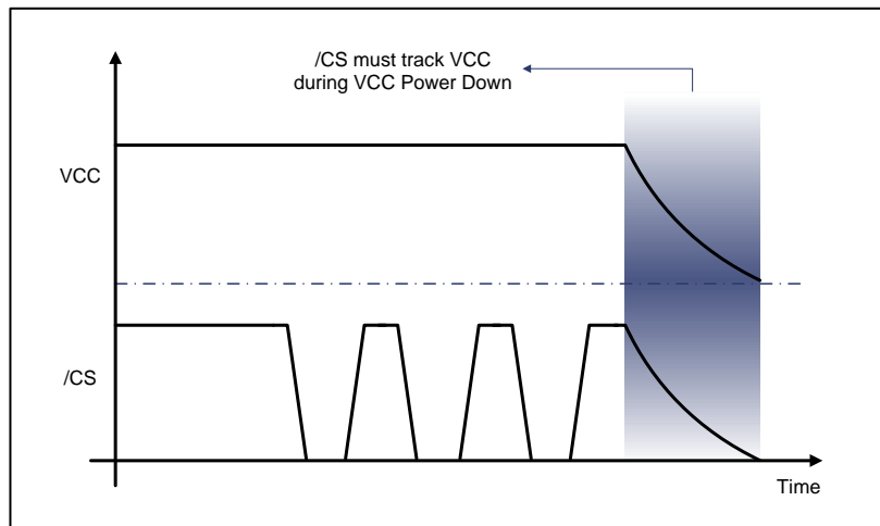
Figure 10-3 Power-Down Timing
