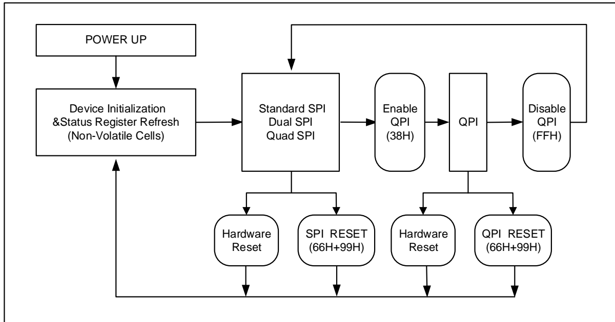
Figure 7-1 XM25QU256D Serial Flash Memory Operation Diagram
