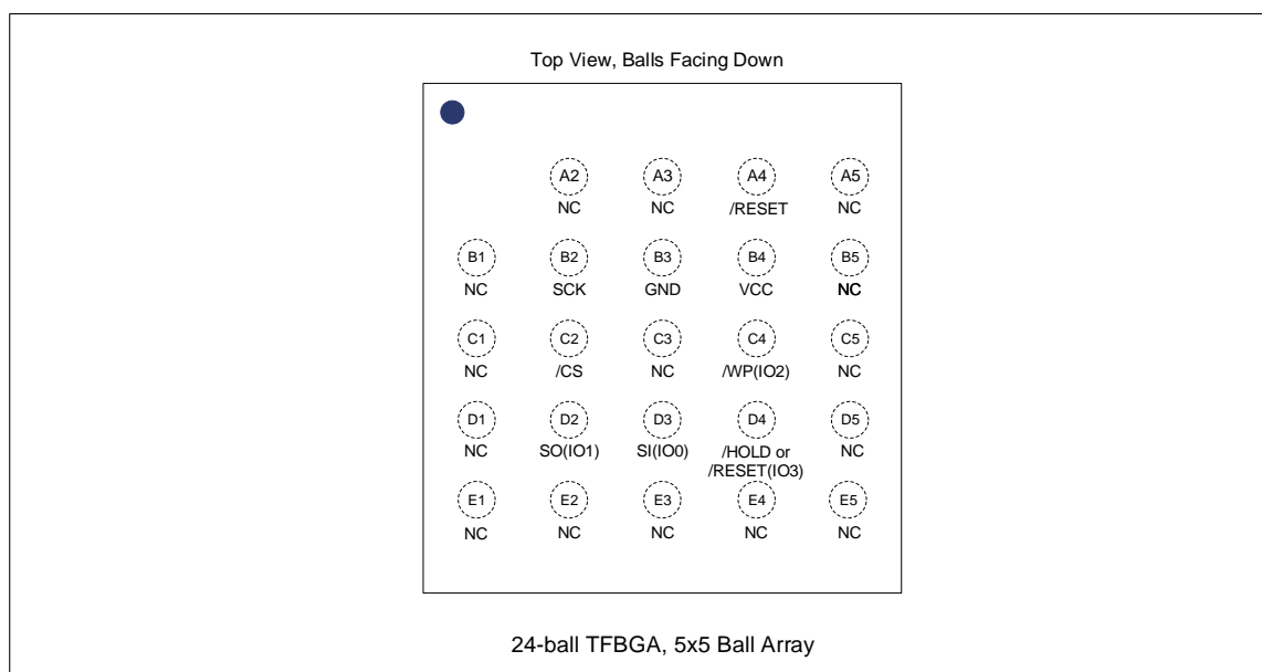
Figure 5-3 24-ball TFBGA 8x6-mm (Package Code B2, 5x5 ball array )
