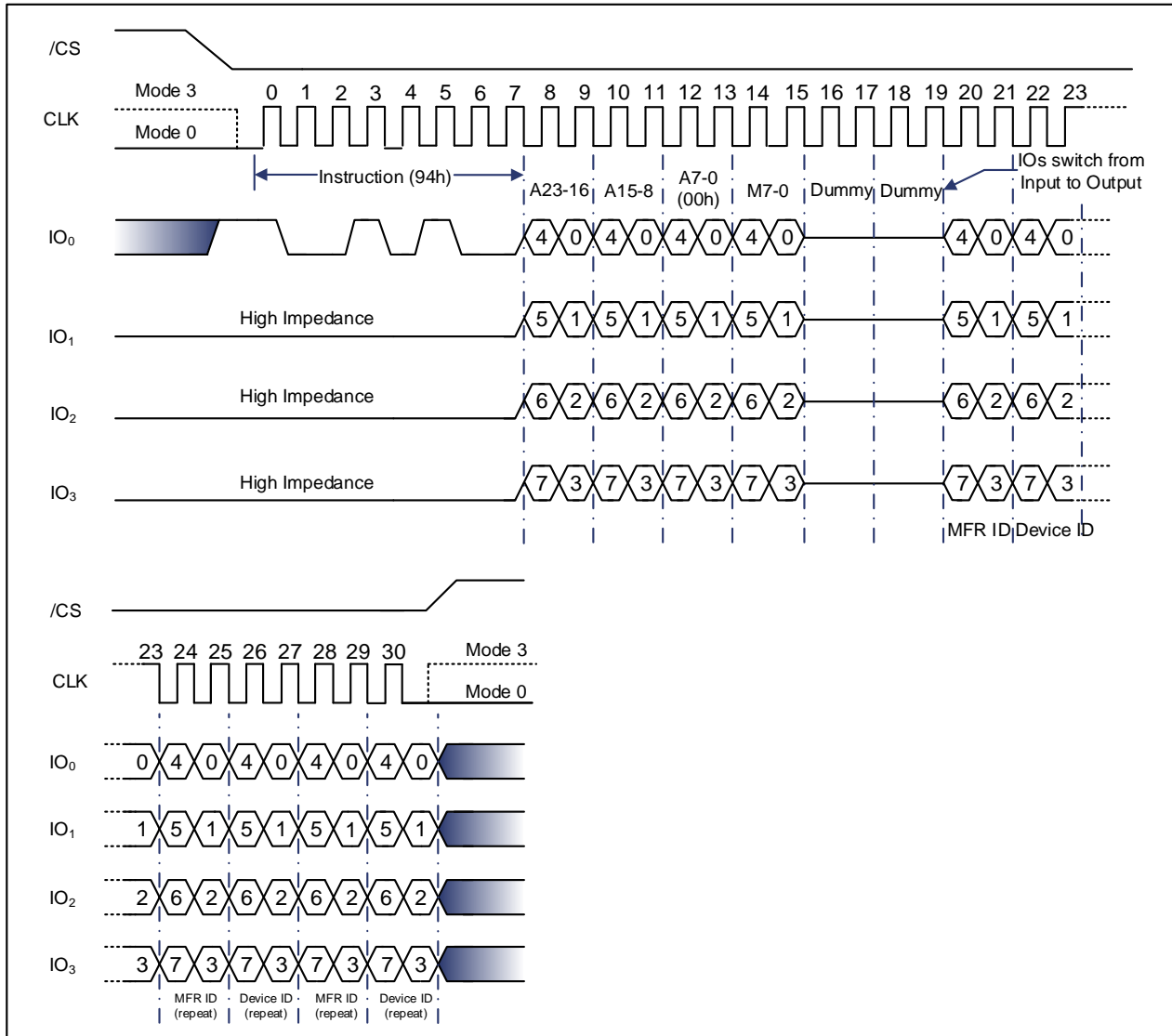
Figure 9-68 Read Manufacturer / Device ID Quad I/O Instruction (SPI Mode only)
