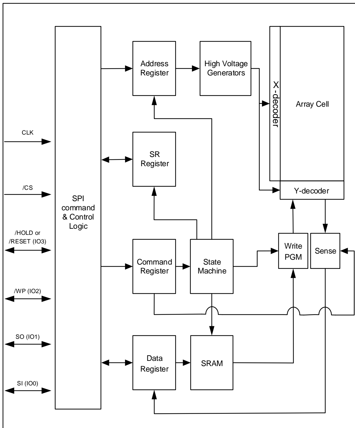
Figure 4-1 XM25QU256D Serial Flash Memory Block Diagram
