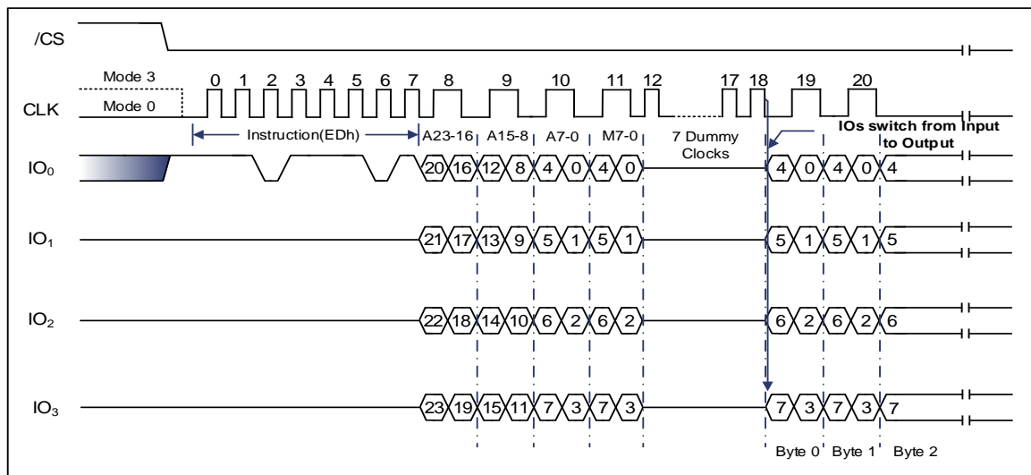
Figure 9-37 DTR Fast Read Quad I/O (Initial instruction or previous M5-4≠10, SPI Mode) 32-Bit Address is required when the device is operating in 4-Byte Address Mode
