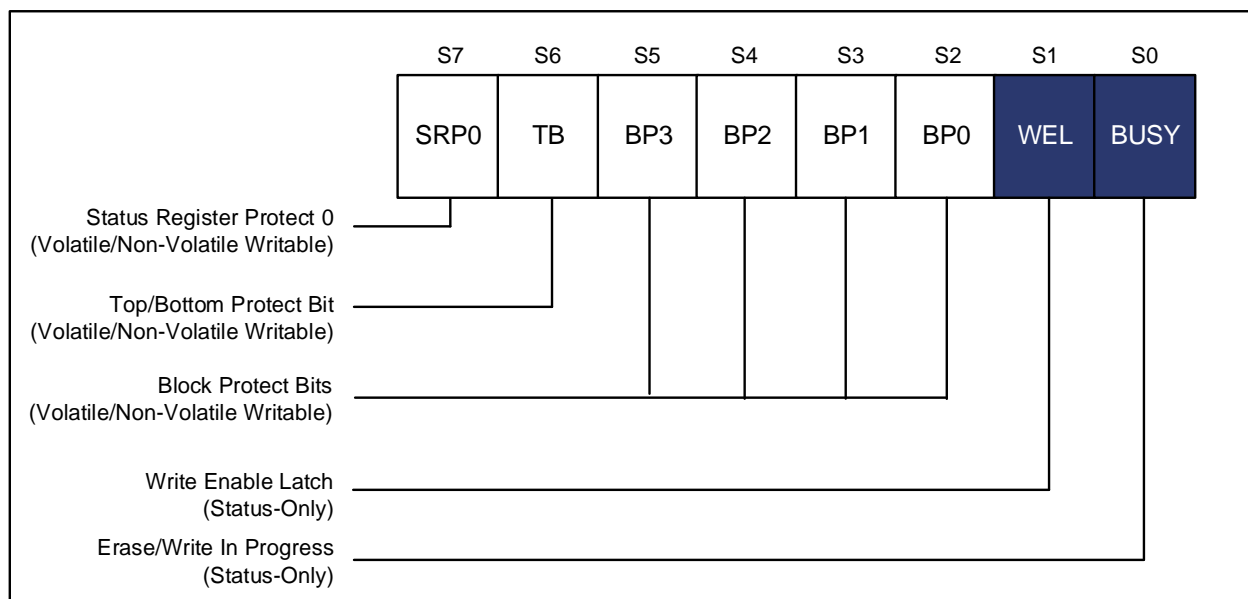
Figure 8-1 Status Register-1
