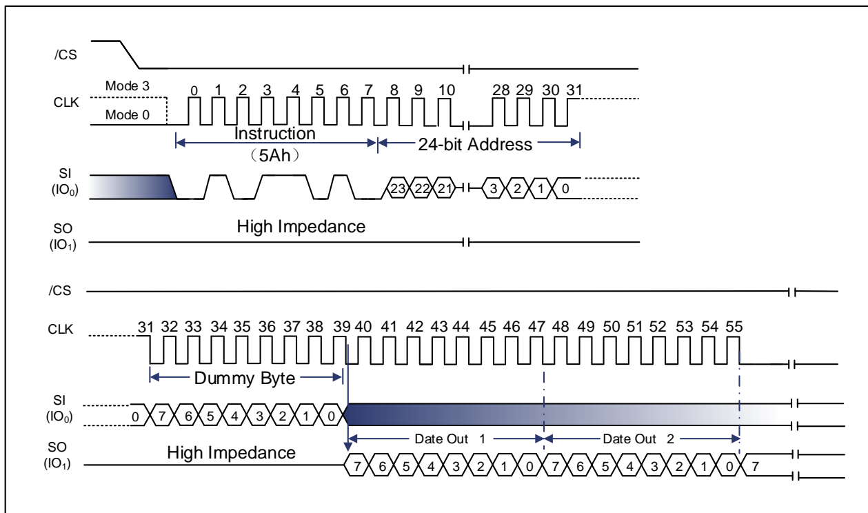
Figure 9-72 Read SFDP Register Instruction Sequence Diagram(Only SPI Mode)
