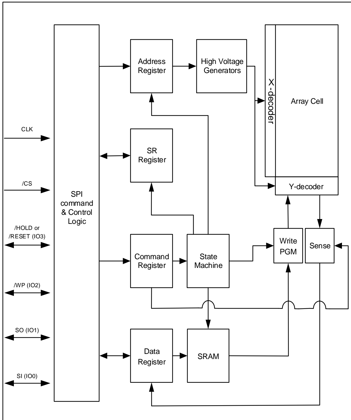
Figure 4-1 XM25QU512D Serial Flash Memory Block Diagram
